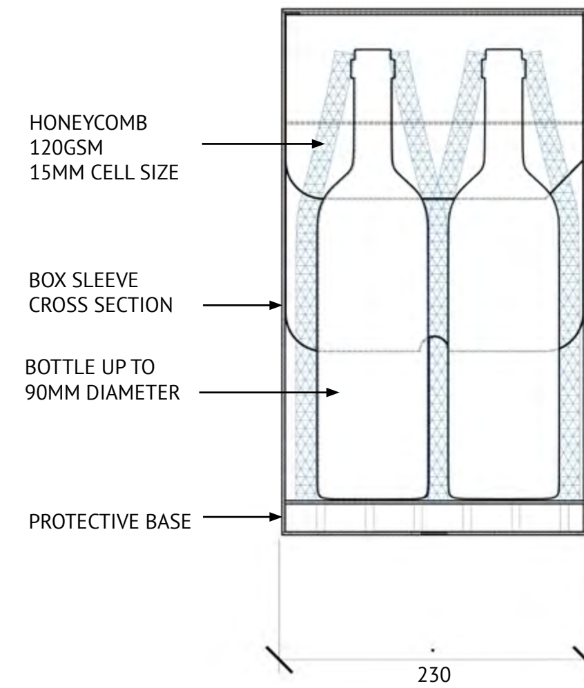
CROSS SECTION VIEW
