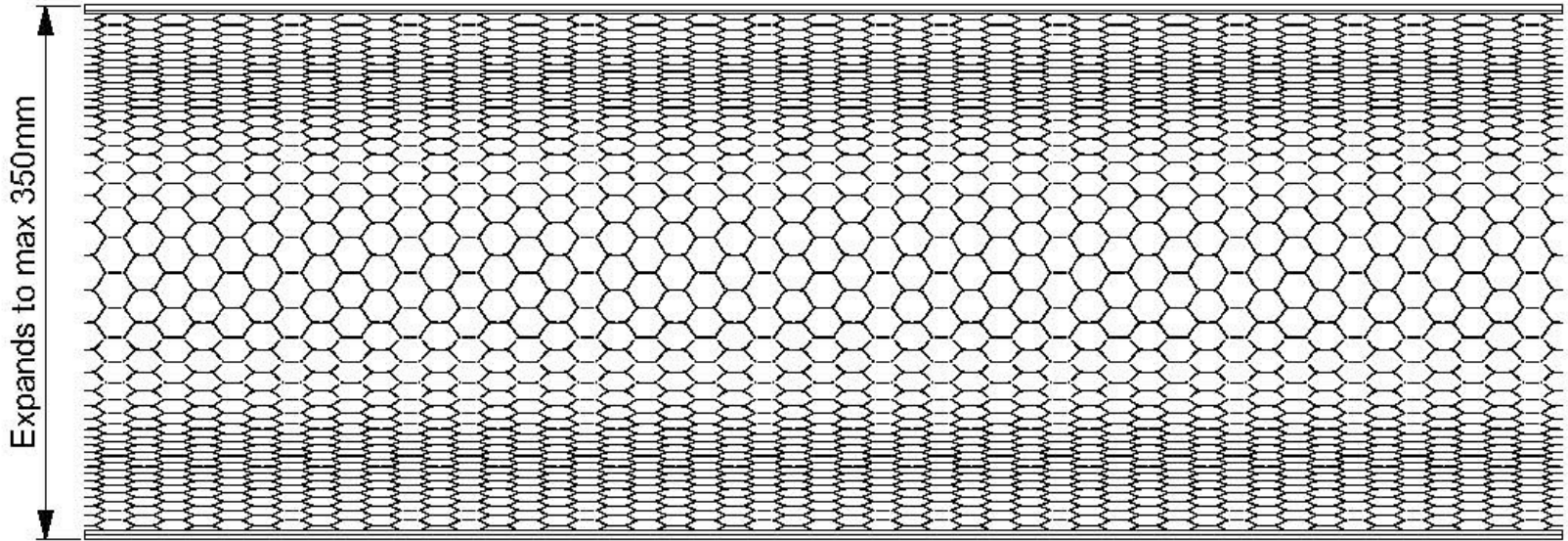
Expanded sleeve
